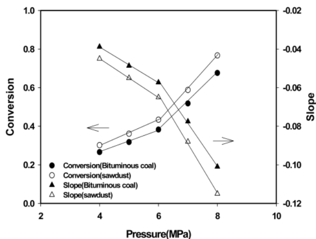
Fig. 4. Conversion and slope of pressure profile with the initial reaction pressure.
